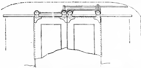
Fig. 2843. DOUBLE SLIDING DOOR FIXTURE. J. L. HOWARD & Co., HARTFORD, CONN.
